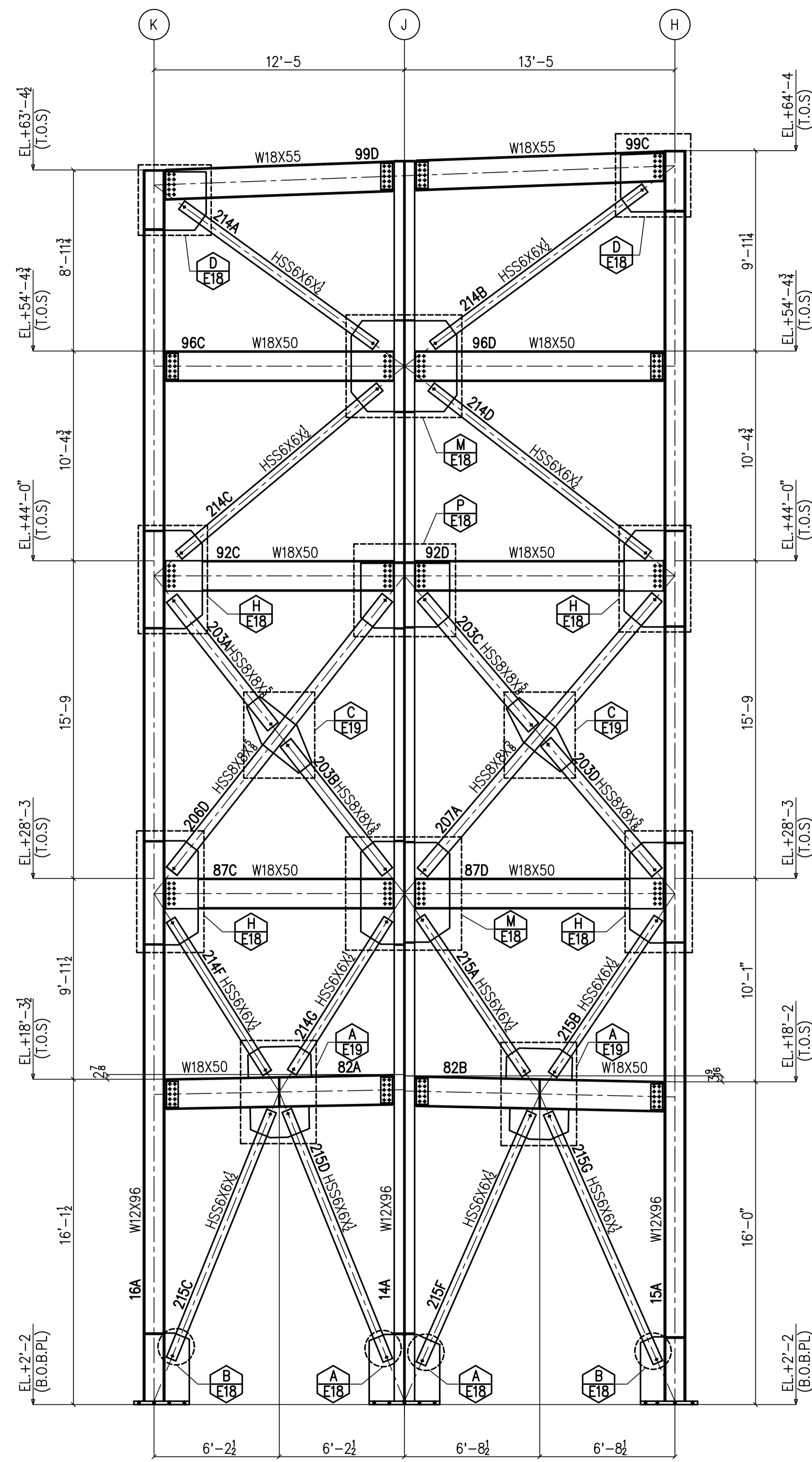
BRACE FRAME ELEV. - GRID LINE '11' ( REF. : 2/S3.1 )
