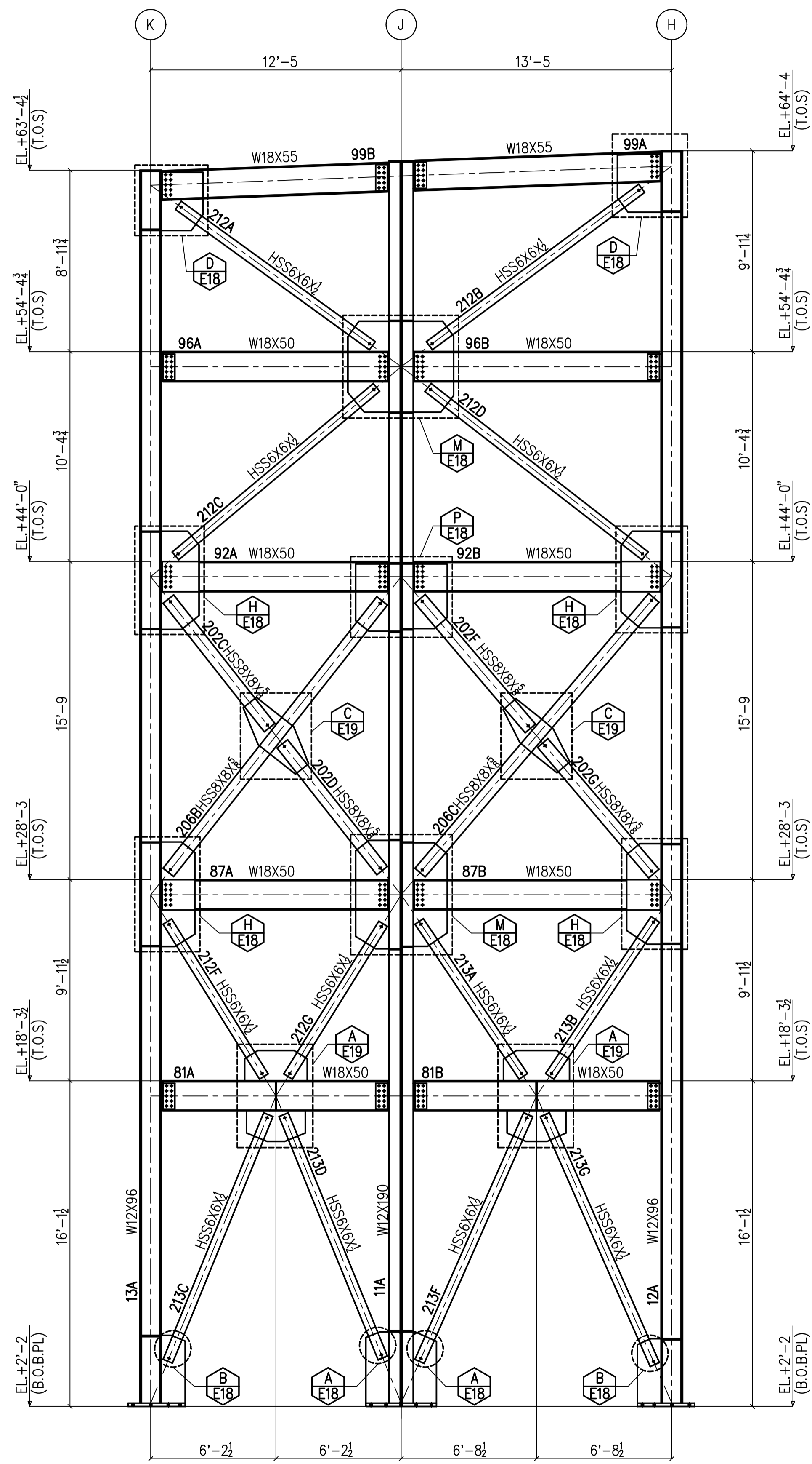
BRACE FRAME ELEV. - GRID LINE '4' ( REF. : 1/S3.1 )
