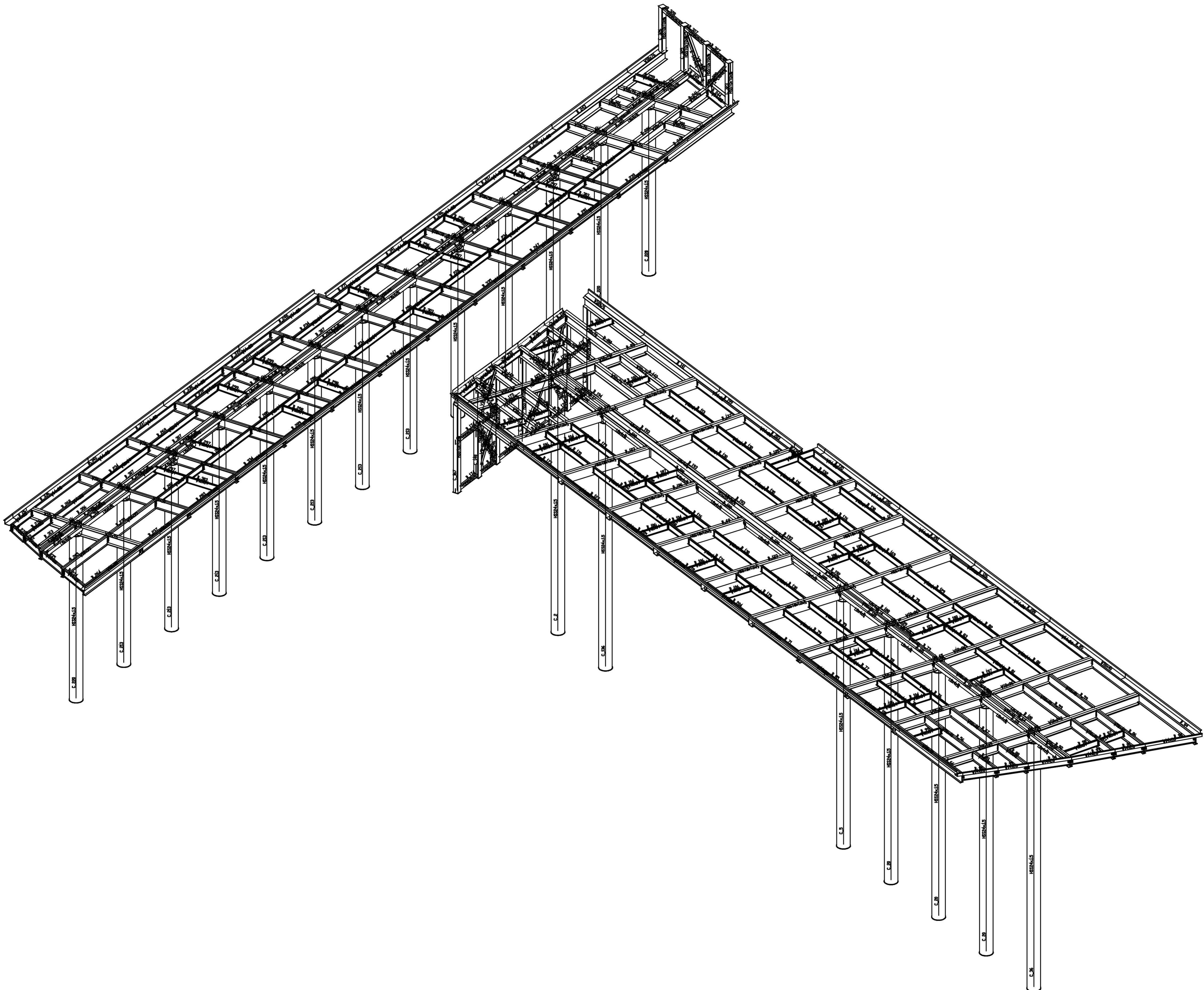
ISOMETRIC VIEW
